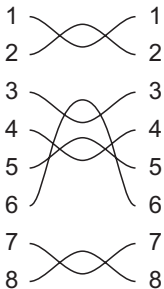
Correct wiring
