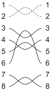
Reversed pair
