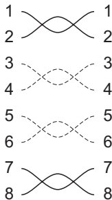
Split pair
