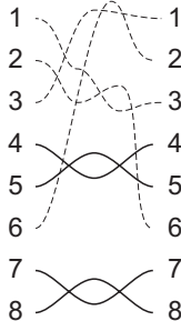
Transposed pair
